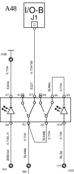
S127 SWITCH, WINDOW HEATER
