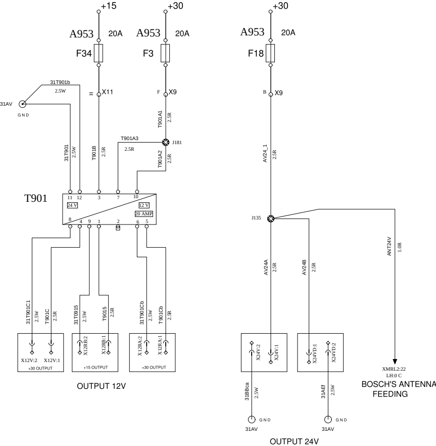
AUDIO AND VIDEO SUPPLY
